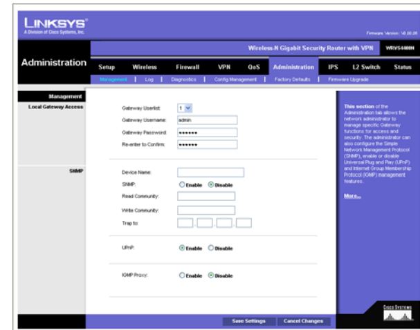
Figure 6-49: Administration - Management
